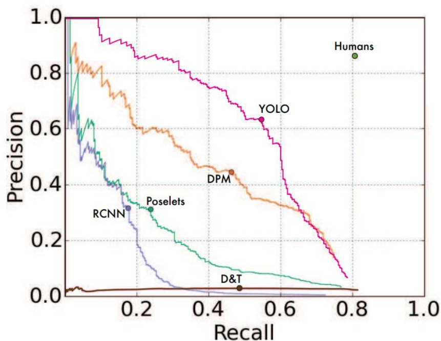
Figure A.4.1 Picasso Dataset precision-recall curves
